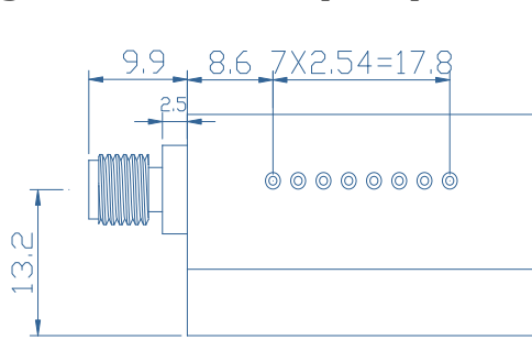
Pin-Out Assignment
